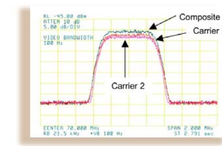
Figure 2: Duplex Link with DoubleTalk Carrier-in-Carrier
